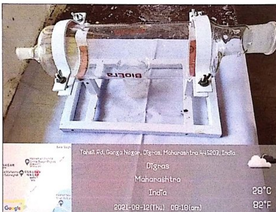
Distillation Assembly
